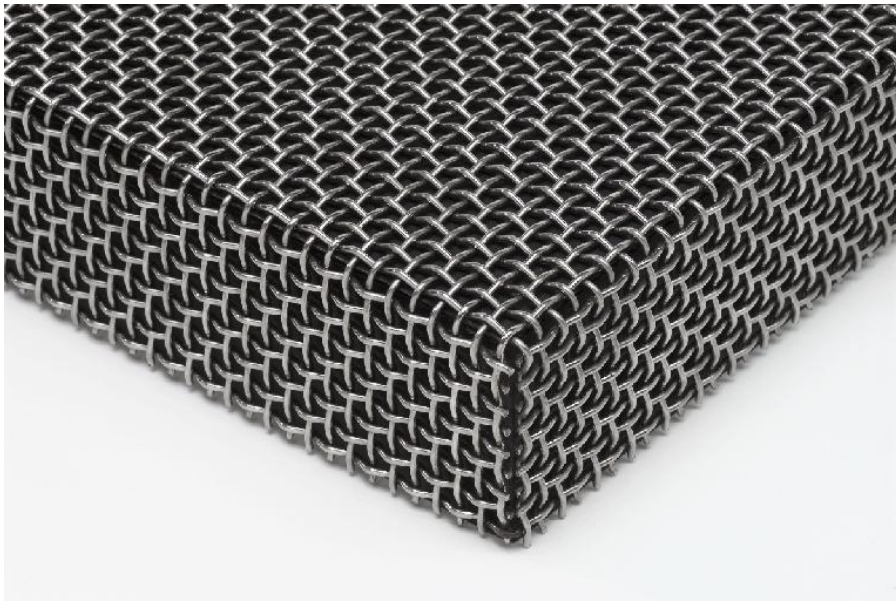
Bent wire cloth elements welded to a frame
