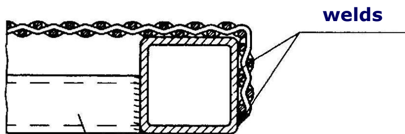
cross bars welded into the frame under pretension
